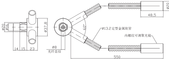
POFC-S7H-1000-F2 GOFC-S7H-1000-F2
