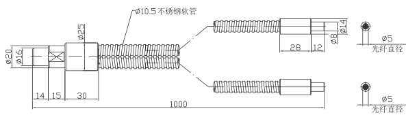
POFC-S8H-1640-FR2 GOFC-S8H-1640-FR2
