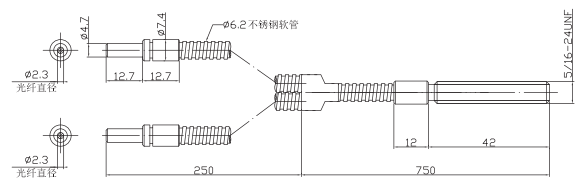
GOFC-S7.8V-500-IB2
