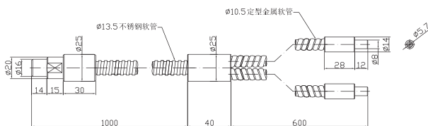
POFC-S8H-1640-FR2 GOFC-S8H-1640-FR2
