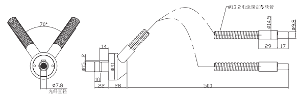
GOFC-S7.8V-500-IB2
