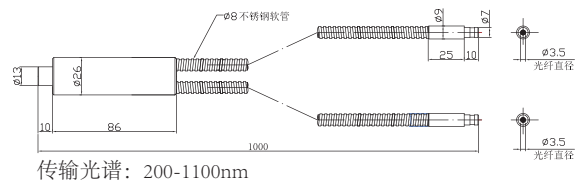
GOFC-S3H-1000-F2H
