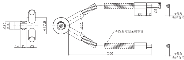
POFC-S8V-500-IT2L GOFC-S8V-500-IT2L
